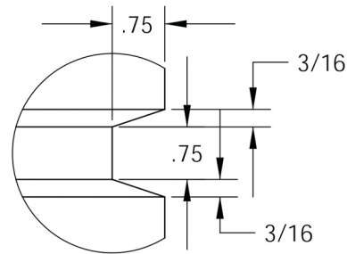
DETAIL B SCALE 1 : 2
