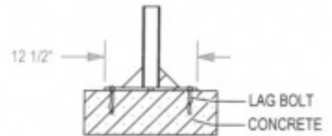
□ SURFACE GUSSET MOUNT (SG)
