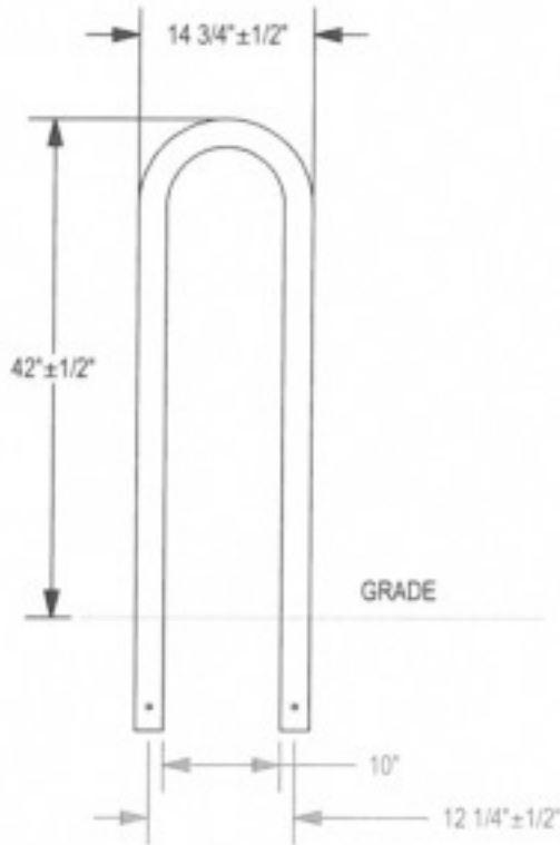
ELEVATION VIEW
