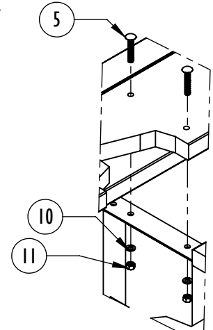
DETAIL L
