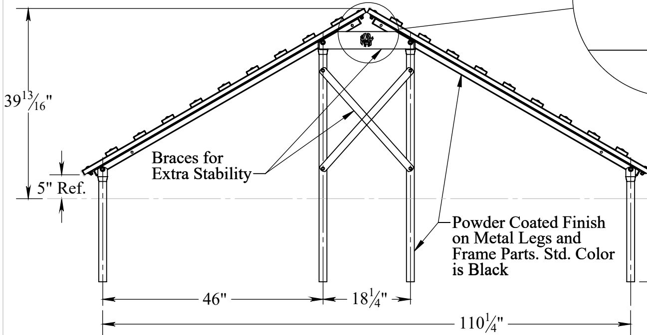
DETAIL F SCALE 1 : 6
